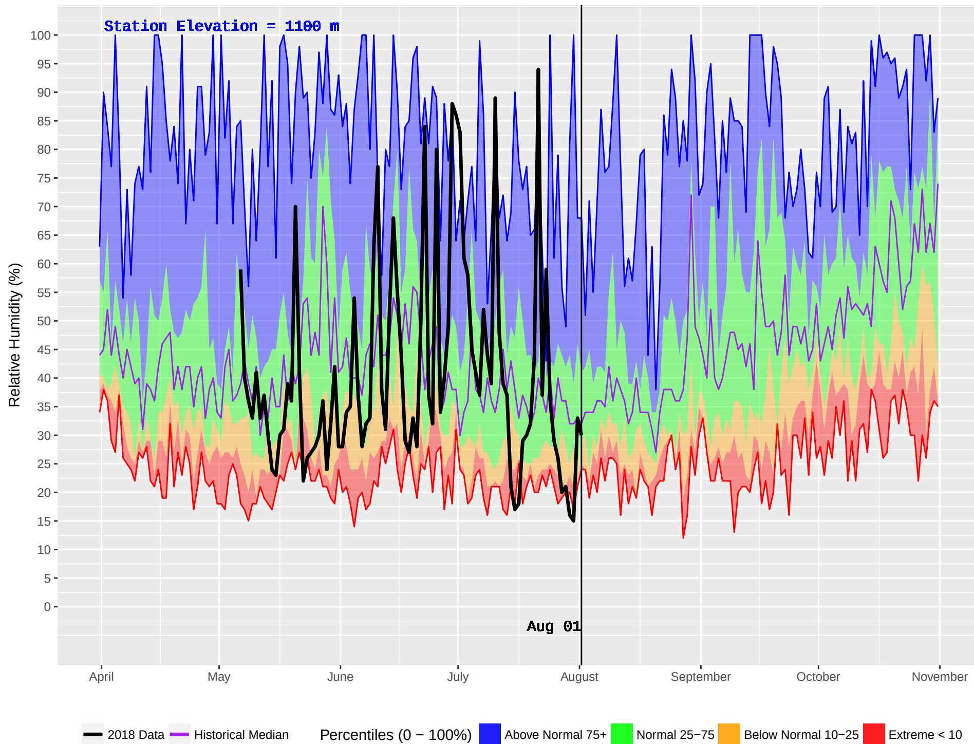
CHURN CREEK (832) : Historical (2003–2016) and Current (2018) Daily Relative Humidity
