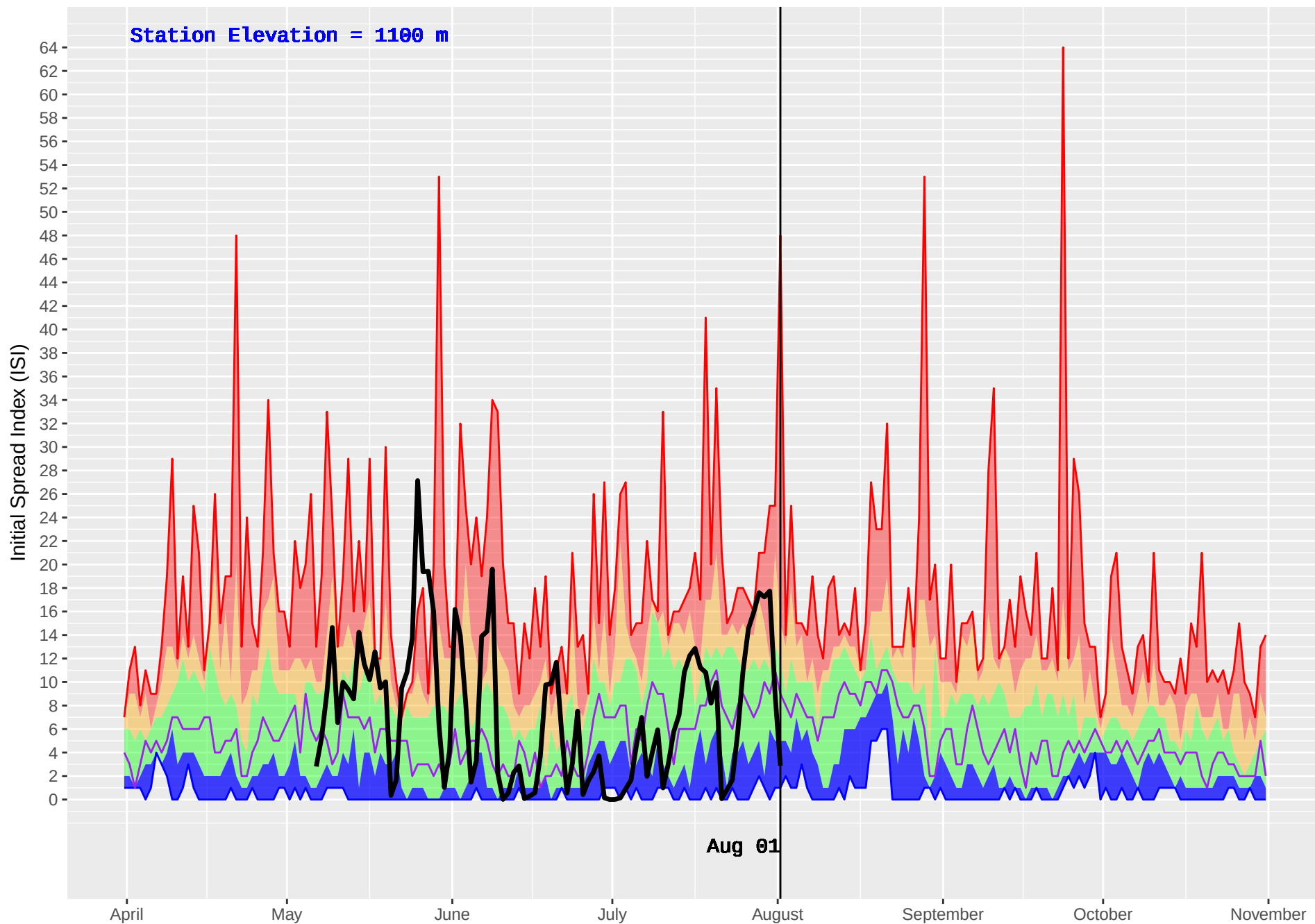
CHURN CREEK (832) : Historical (2003–2016) and Current (2018) Daily Initial Spread Index (ISI)
